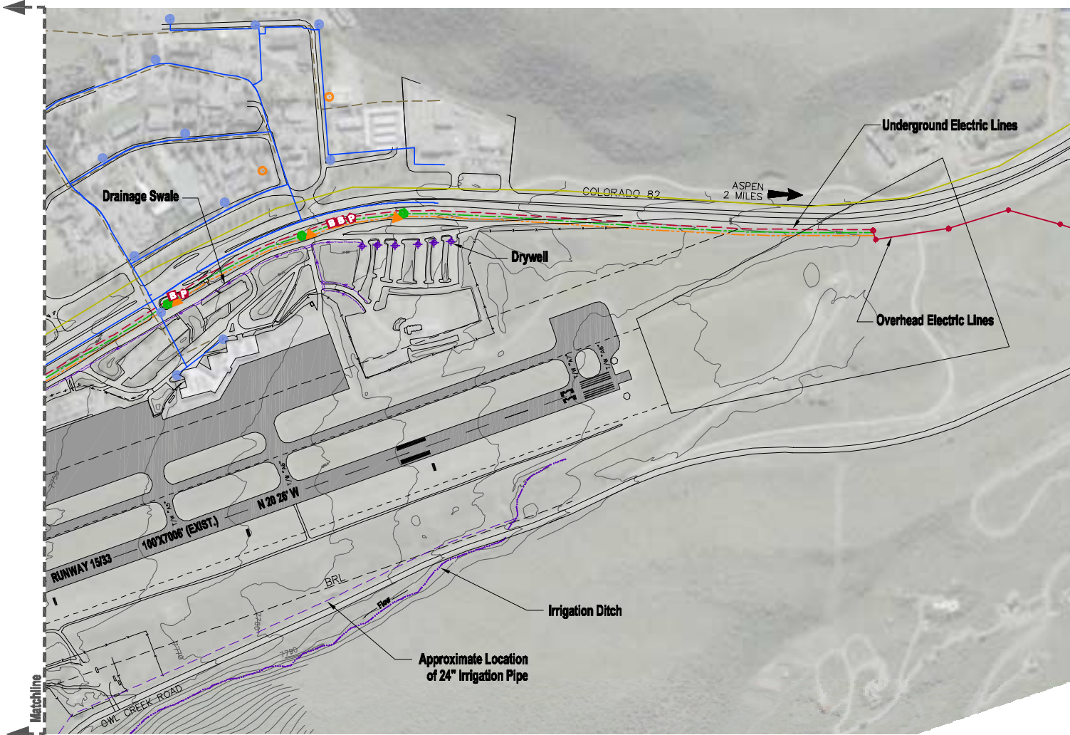
▶ FIGURE A6 Existing Utility Locations - South
